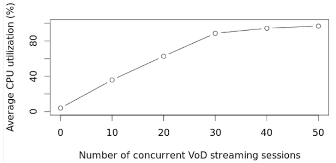
Fig. 3. Average CPU utilisation across cores versus the number of concurrent VoD streaming sessions
